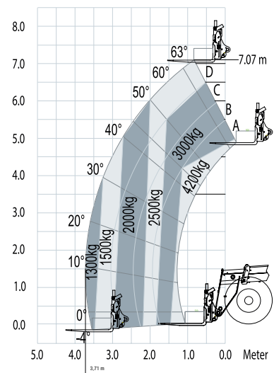
STH1133 – OUTRIGGERS DOWN
